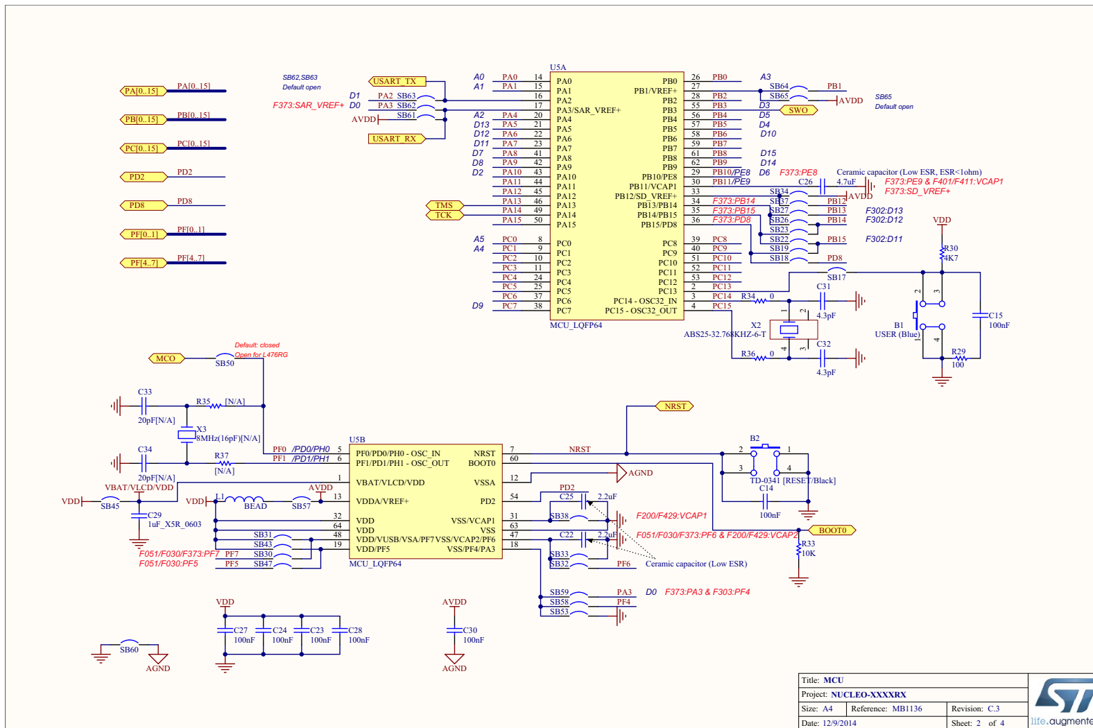
Figure 25. Electrical schematics (2/4)
