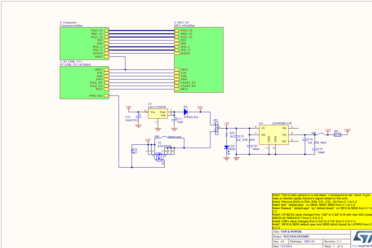
Figure 24. Electrical schematics (1/4)
