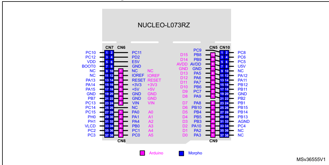
Figure 20. NUCLEO-L073RZ
