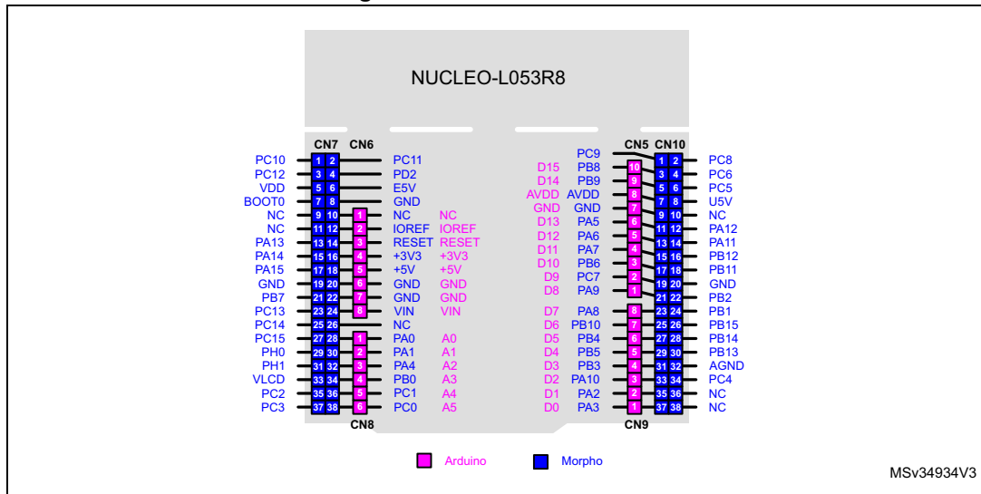
Figure 19. NUCLEO-L053R8
