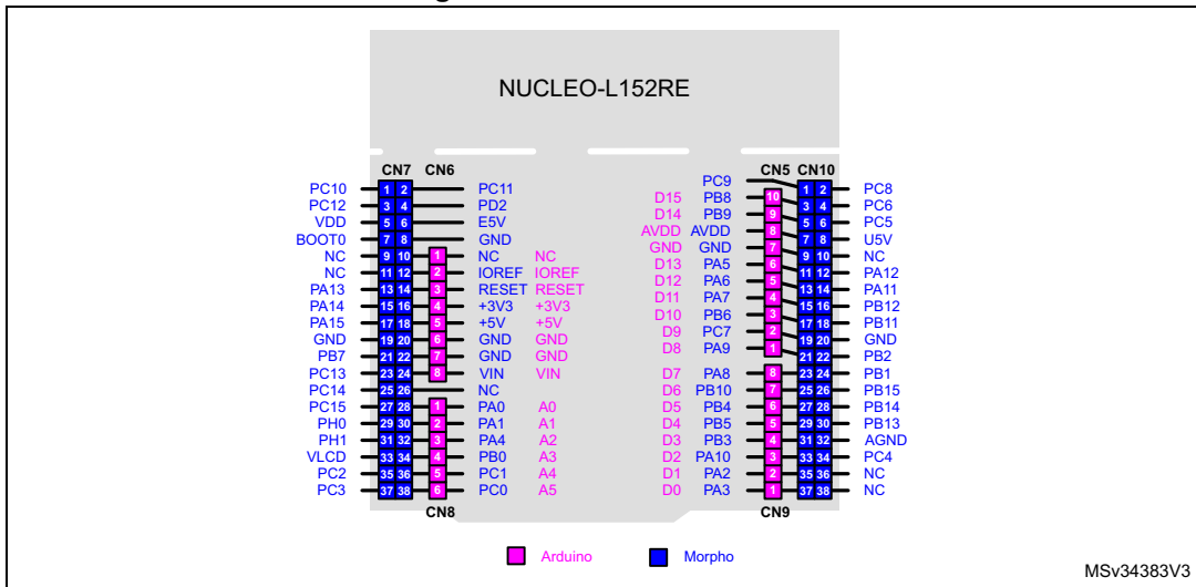
Figure 21. NUCLEO-L152RE
