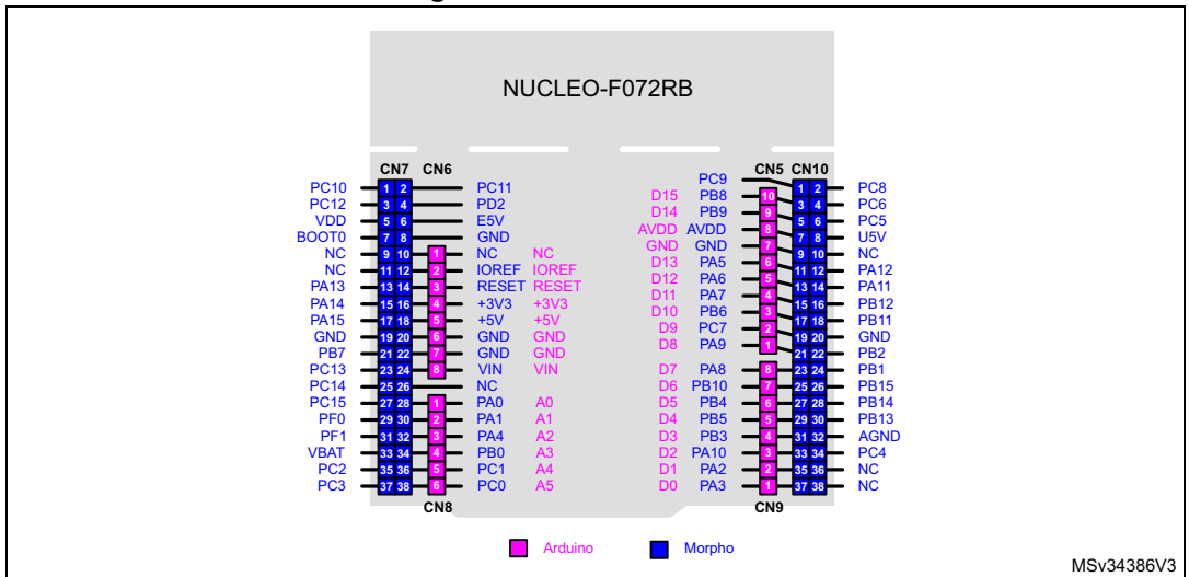
Figure 11. NUCLEO-F072RB
