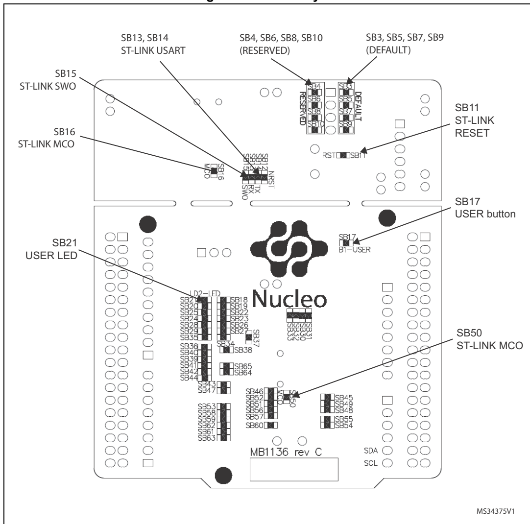
Figure 4. Bottom layout
