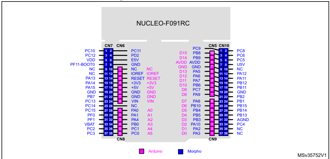
Figure 12. NUCLEO-F091RC
